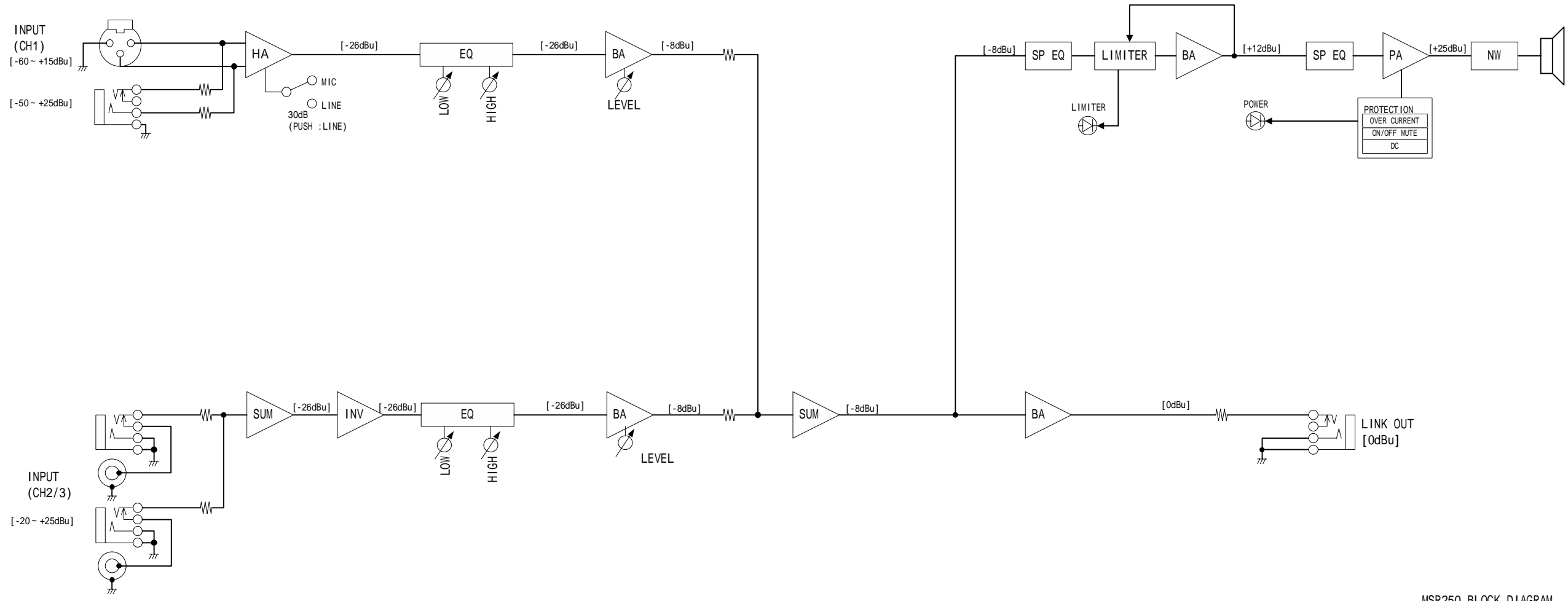
MSR250 BLOCK DIAGRAM
